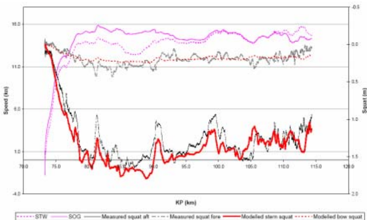
Figure 8: Squat validation results for E-Class Maersk container vessel.
