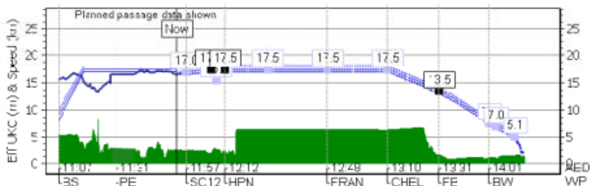
Figure 10: Example of InTransit for Weser DUKC®
