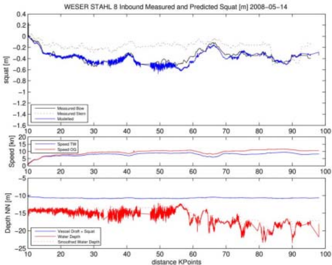
Figure 9: Squat validation results Weser Stahl (LBP ~220, Beam~32)
